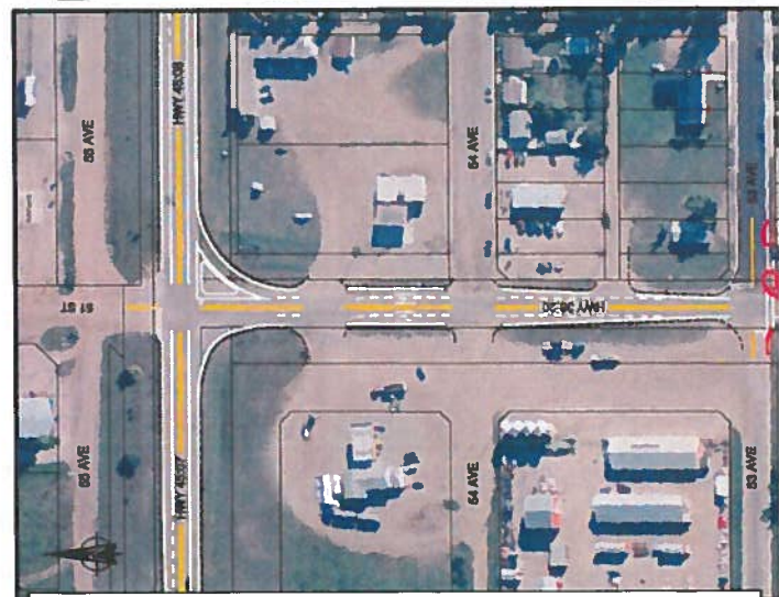
Figure 2. Diagram illustrating the intersection improvements at Highway 36 and Highway 45
